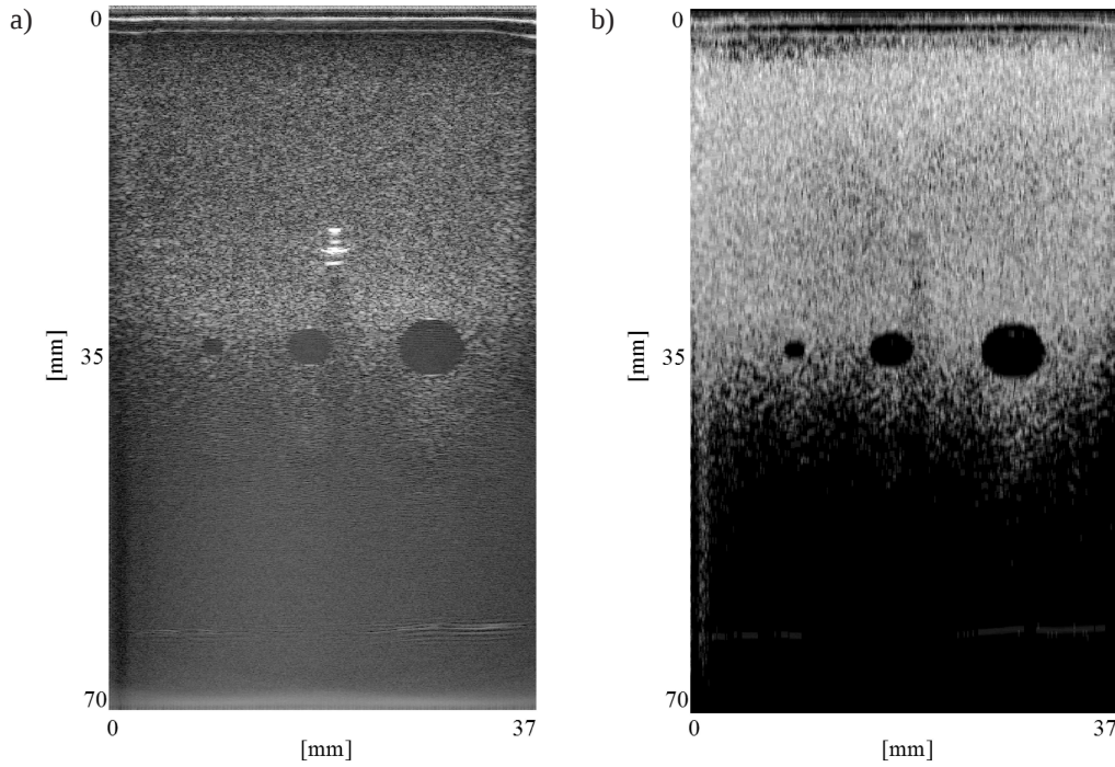
Fig. 1. B-mode scan (a), and frequency mapping (b) of the tissue phantom.
