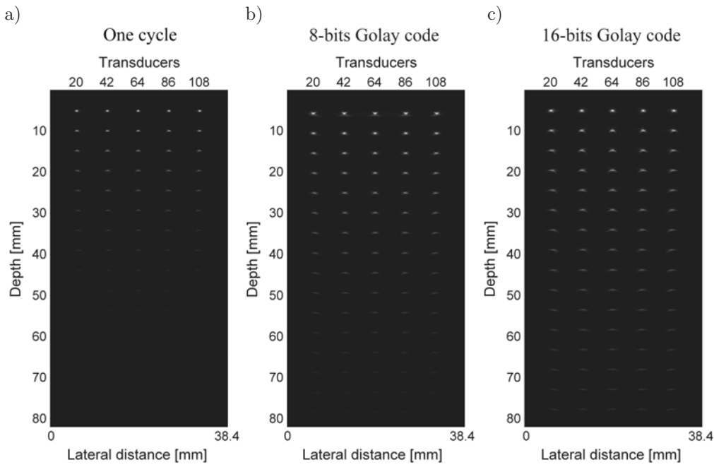
Fig. 5. Comparison of 2D ultrasound images obtained by computer simulation for 128-element linear array using: a) one cycle; b) 8-bits Golay sequences; c) 16-bits Golay sequences.
