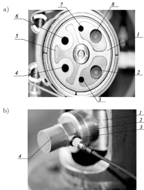
Fig. 4. The location and method of fixing the transducer: a) the view from weight top (Fig. 3): 1 – measuring position, 2 and 8 – holes for dowels, 3 and 7 – cooling channels, 4 and 6 – fuel channels; b) the place of fixing the transducer: 1 – atomizer, 2 – profiled connector, 3 – fixing magnesium, 4 – transducer (sensor).
