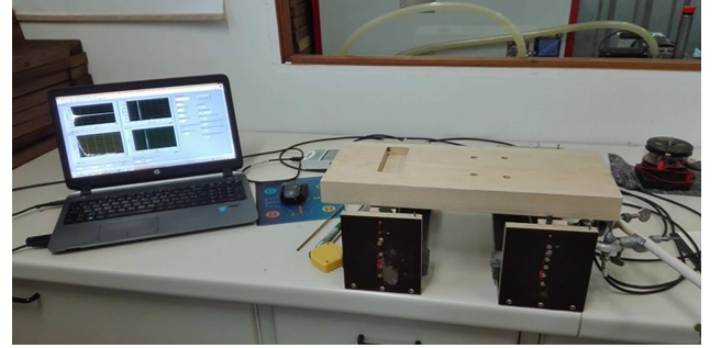
Fig. 3. Experimental setup of free-free flexural vibration measurements of wood elements.
