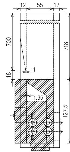
Fig. 2. Side view of the experimental pipe. The lengths are in millimeters.
