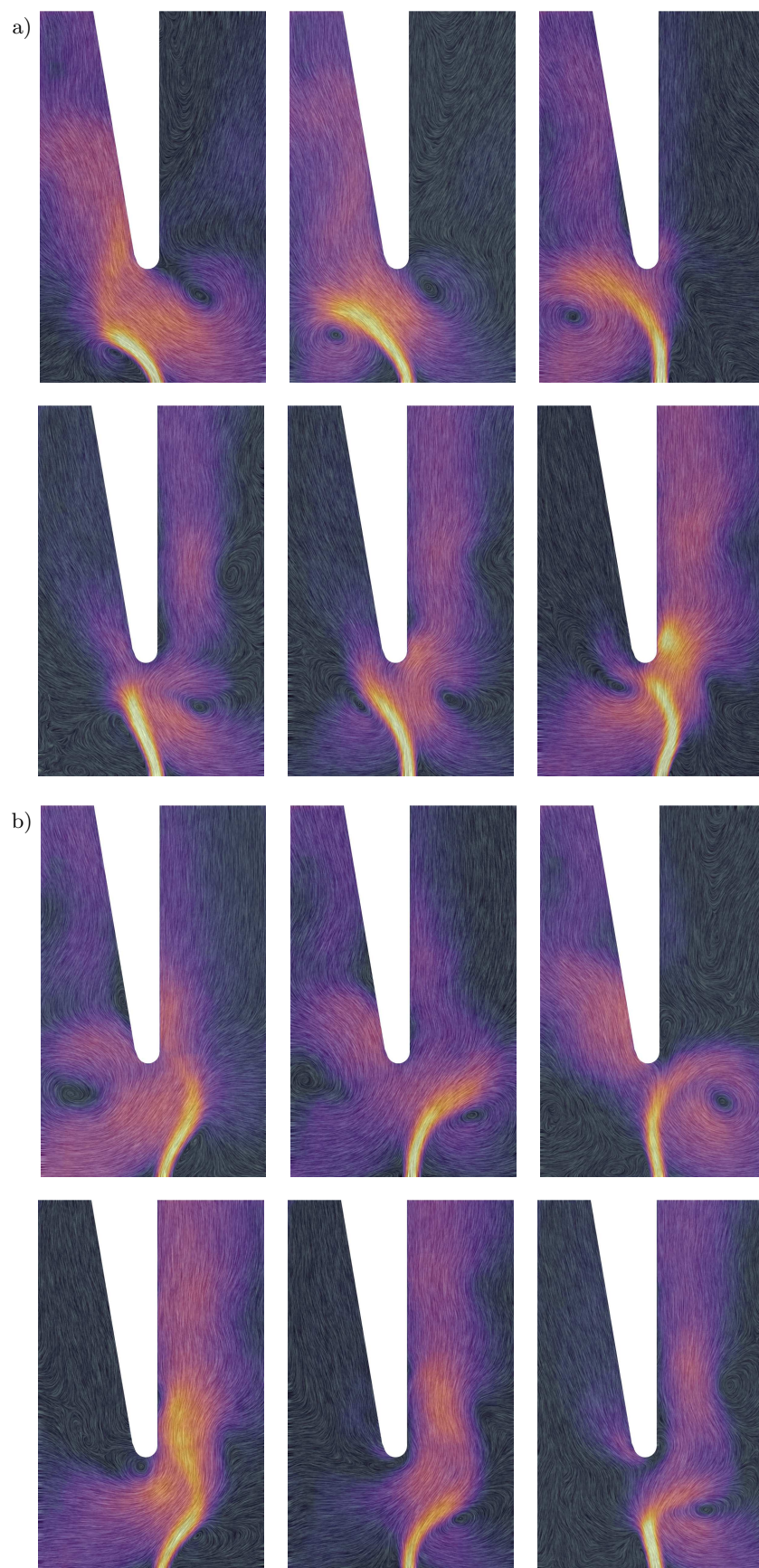
Fig. 5. Comparison of the phases 1, 7, 13 (a) and 19, 25, 31 (b). Within the sextuplets the closed configuration is always at the top and the open at the bottom.
