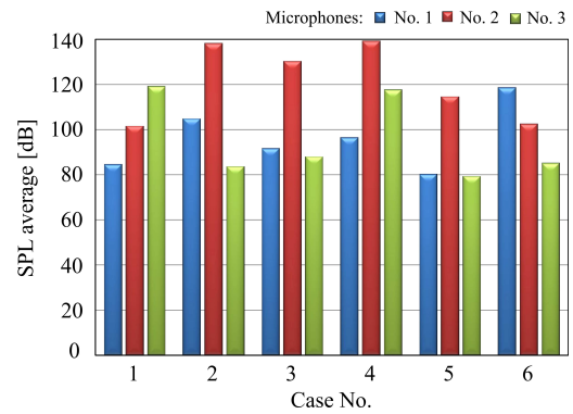
Fig. 14. The average sound pressure level in different cases of input and outlet element relative to the position of the plenum chamber.
