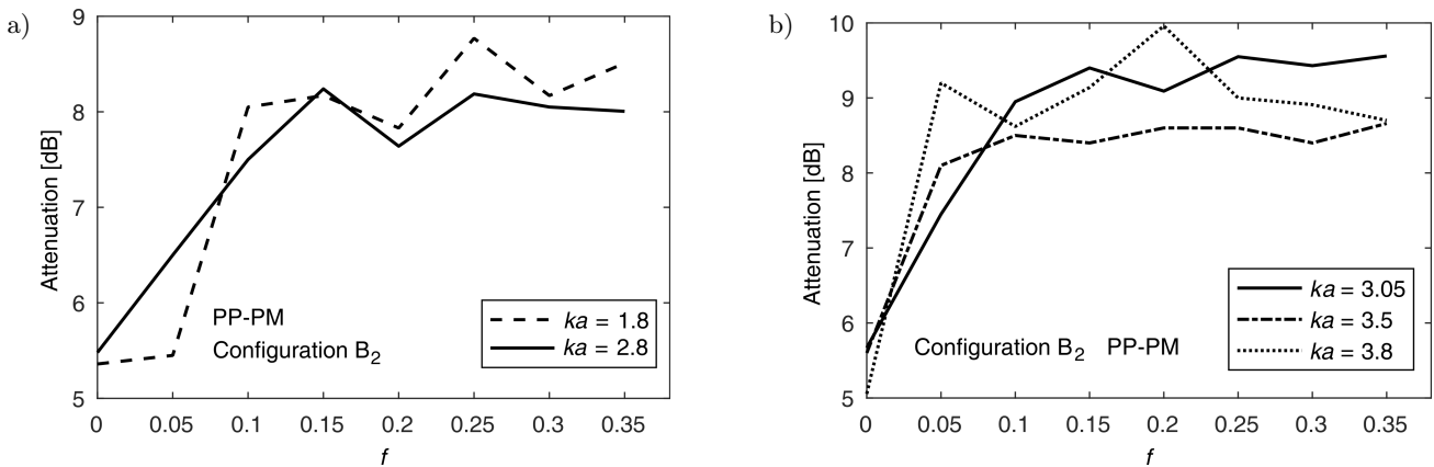
Fig. 9. Acoustic power attenuation versus progressive part f of configuration B 2 treated by PP-PM liner model for several ka (a) and (b).
