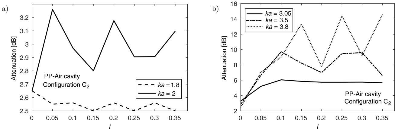
Fig. 10. Acoustic power attenuation versus progressive part f of configuration C 2 treated by PP-Air cavity liner model for several ka (a) and (b).
