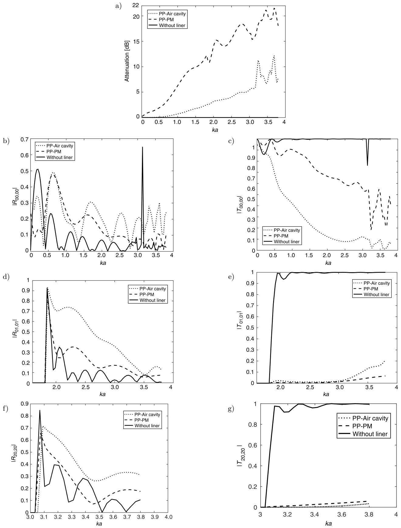
Fig. 7. Comparison of the acoustic behavior (acoustic power attenuation and scattering matrix coefficients in the presence of (0, 0) mode (b, c), (1, 0) mode (d, e) and (2, 0), mode (f, g)) versus ka between two acoustic liners' models: PP-PM and PP-Air cavity of configuration C_2 .
