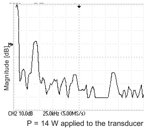
Fig. 12. Output signal spectrum achieved in a multi-mode coupler system when the power P = 14 \text{ W} is applied to the transducer (the power for which fringes were achieved).
