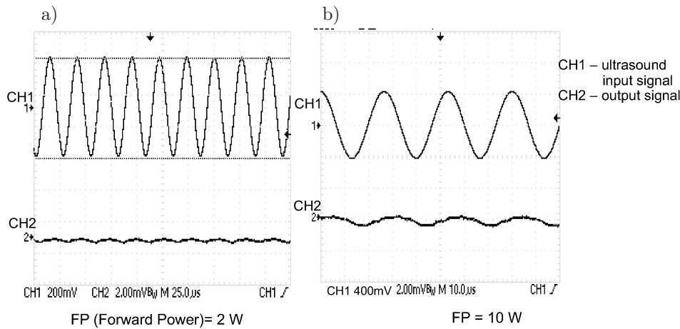
Fig. 5. Temporary courses achieved in a multi-mode coupler system when the power applied to the transducer is: a) 2 W, b) 10 W.
