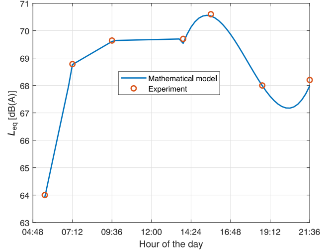
Fig. 6. Comparison of the mathematical model with experimental data of the equivalent noise level during the day for Yaroslav Mudryj Street.
