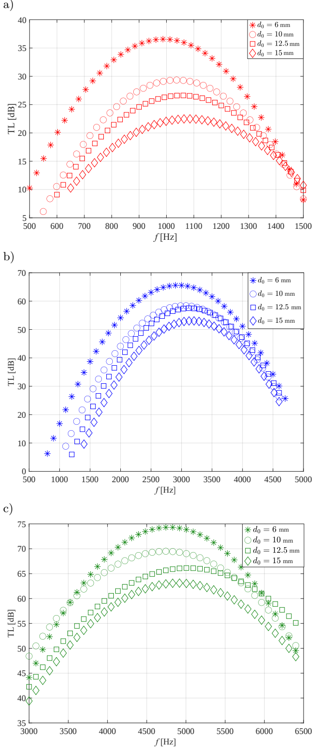
Fig. 16. Effect of the diameter of the transverse partition d_0 = \{6, 10, 12.5, 15\} mm, h = 5 mm, between D-ECs on the TL for selected frequencies: a) 1000 Hz, b) 3000 Hz, c) 5000 Hz.
