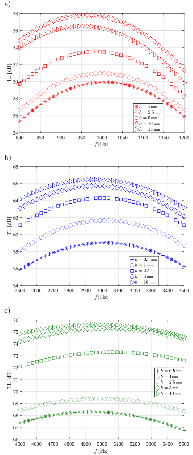
Fig. 15. Effect of the transverse partition width h [mm], d_0 = 6 mm, between D-ECs on the TL for selected frequencies: a) 1000 Hz, b) 3000 Hz, c) 5000 Hz.
