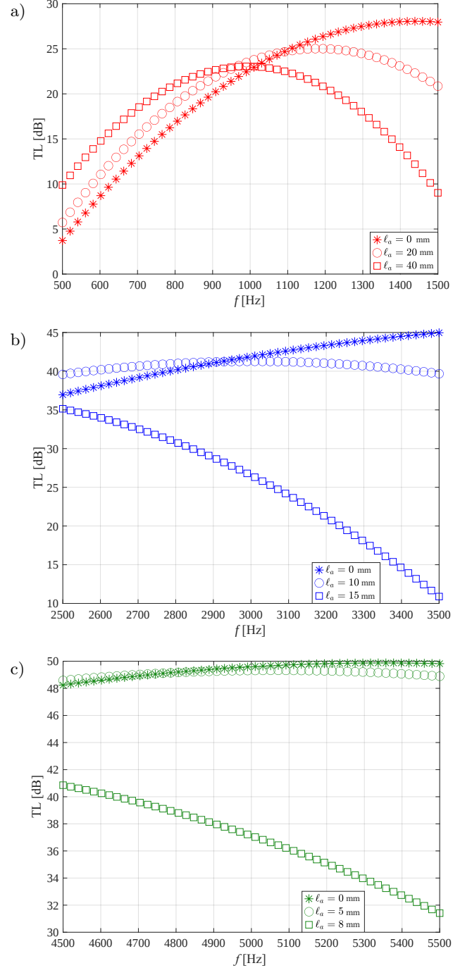
Fig. 3. Influence of different \ell_a values on the maximum TL at selected frequencies: a) 1000 Hz, b) 3000 Hz, c) 5000 Hz.
