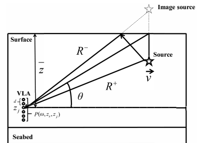
Fig. 1. Diagram of the source and vertical line array (VLA) geometry.
