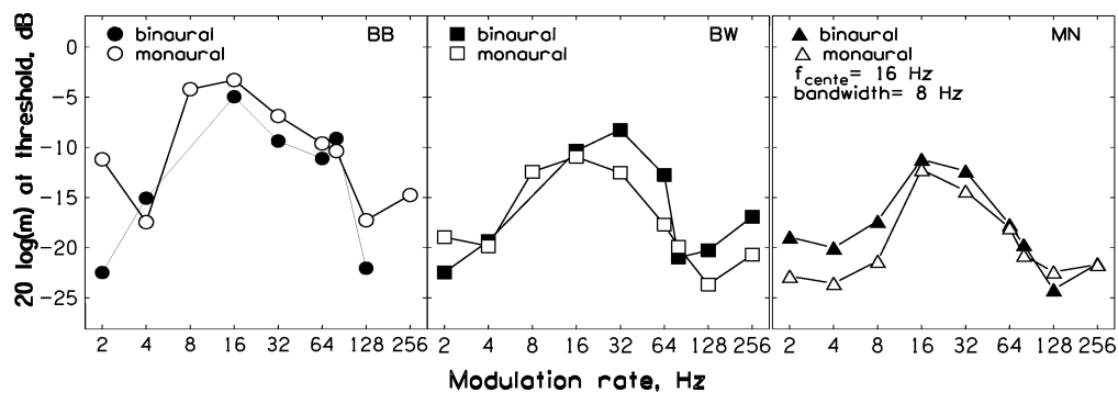
Fig. 2. Amplitude modulation depth expressed as 20 \log(m) at the detection threshold (ordinate) as a function of the modulation rate (abscissa). Low-Noise-Noise (LNN) at the center frequency of 16 Hz and the bandwidth of 8 Hz was used as a masker.
