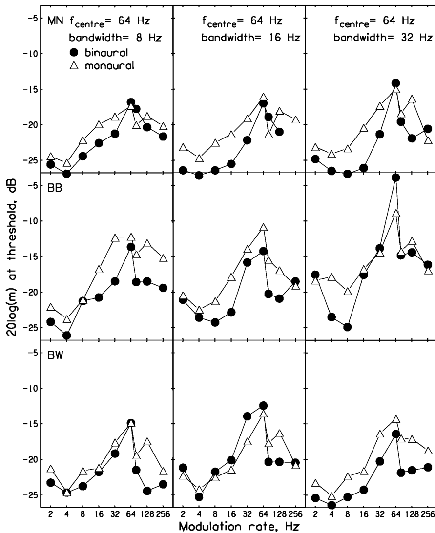
Fig. 1. Amplitude modulation depth expressed as 20 \log(m) at the detection threshold (ordinate) as a function of the modulation rate (abscissa). Low-Noise-Noise (LNN) at the center frequency of 64 Hz and the bandwidth of 8, 16 or 32 Hz was used as a masker.
