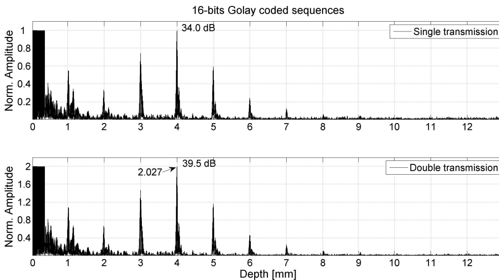
Fig. 5. The centre RF-lines of the tissue phantom obtained by single transmission (top) and double transmission (bottom) of 16-bits Golay sequences.
