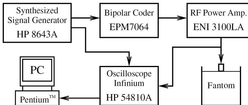
Fig. 3. Diagram of experimental setup.
