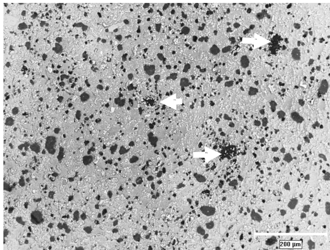
Fig. 5. Typical structure of the sample loaded up to the advanced subcritical level. Black, crushed out parts of glassy-mullite precipitates, quartz grains, cullet fragments and damaged agglomerates of corundum grains (marked by arrows) are visible. Black places comprise together 13 percent of the surface.
