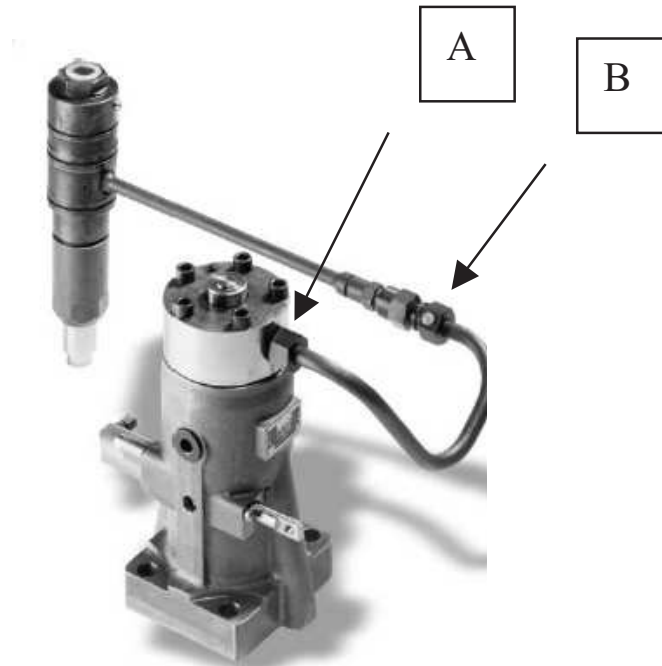
Fig. 2. Placement of the acoustic sensor for monitoring the signals generated by the fuel pump (A) and the injector (B).
