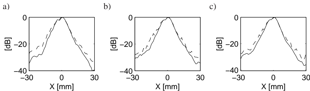
Fig. 5. Changes of pressure on line sheer to the beam, 50 mm away from the transducer for chirp (a), Barker code (b) and Golay code (c). Solid and dashed line denotes the compressed and non-compressed beam respectively.
