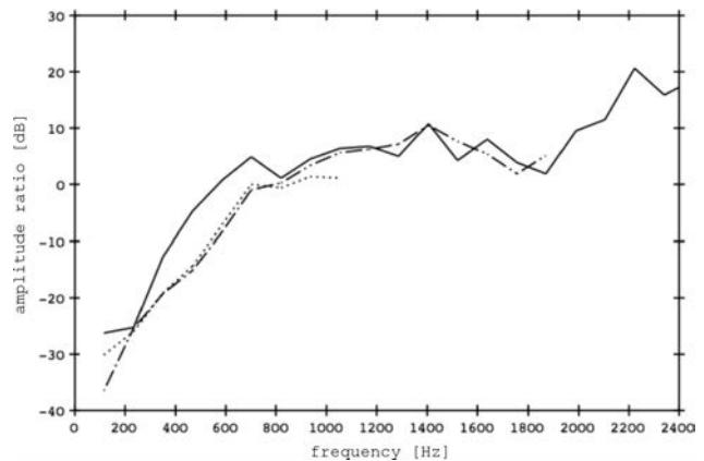
Fig. 1. Trombone transfer functions made under performance conditions for B_2^b ( f_1 \approx 117 Hz) tones played at dynamics pp (dotted curve), mf (dash-dot curve), and ff (solid curve). Curves are discontinued when input harmonic falls below a noise floor.
