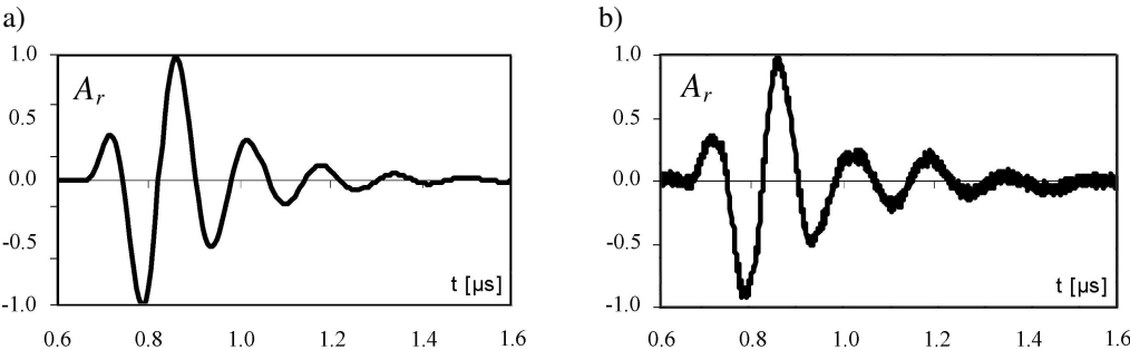
Fig. 3. a) The assumed normalized mechanical stimulation; b) the measured normalized mechanical stimulation, A_r = P/P_0 , where P – pressure, P_0 = 0.25 MPa.
