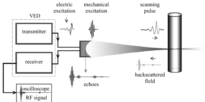
Fig. 1. Experimental setup.
