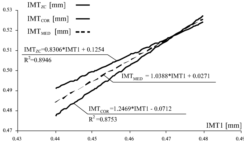
Fig. 3. Numerical experiment. Comparison of the methods used for IMT examination. IMT1 – true values. \text{IMT}_{\text{ZC}} – results obtained on the basis of the zero-crossing method \text{IMT}_{\text{COR}} – results obtained on the basis of the correlation method. \text{IMT}_{\text{MED}} – mean values – dashed line.
