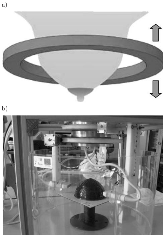
Fig. 1. a) Concept for breast imaging in real-time based on a circular array with thousands of elements, b) experimental arrangement with mechanically rotated conventional arrays.
